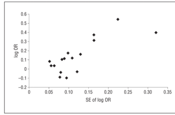
Figure 1. Funnel plot of single-nucleotide polymorphism 8 (white and Asian data sets). OR indicates odds ratio.
